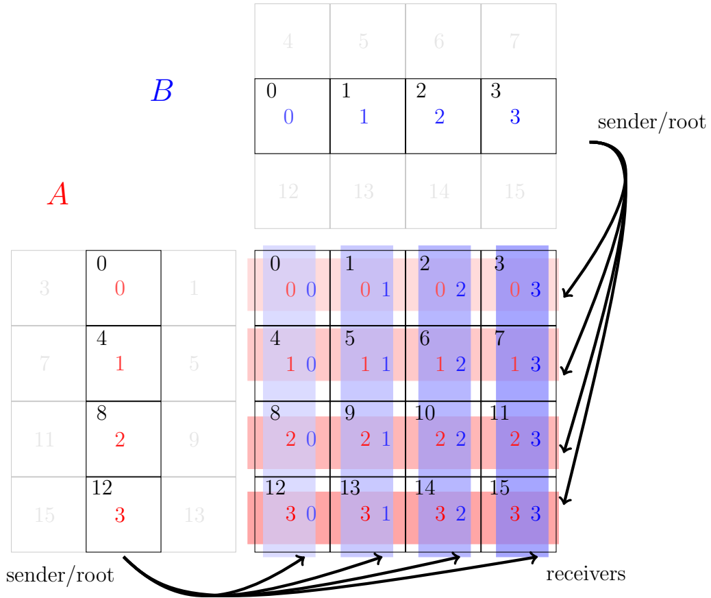
Figure 3: Communication patterns on a 4 \times 4 grid for the transmission of one column of A and one row of B
